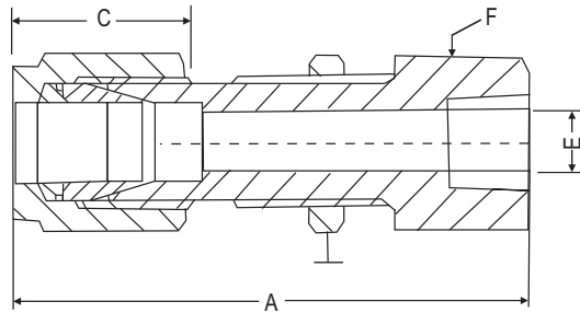
Dimensional Details :
